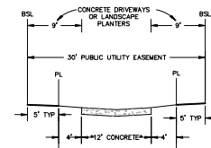
TN-12 (TYPICAL NEIGHBORHOOD ALLEY SECTION)
