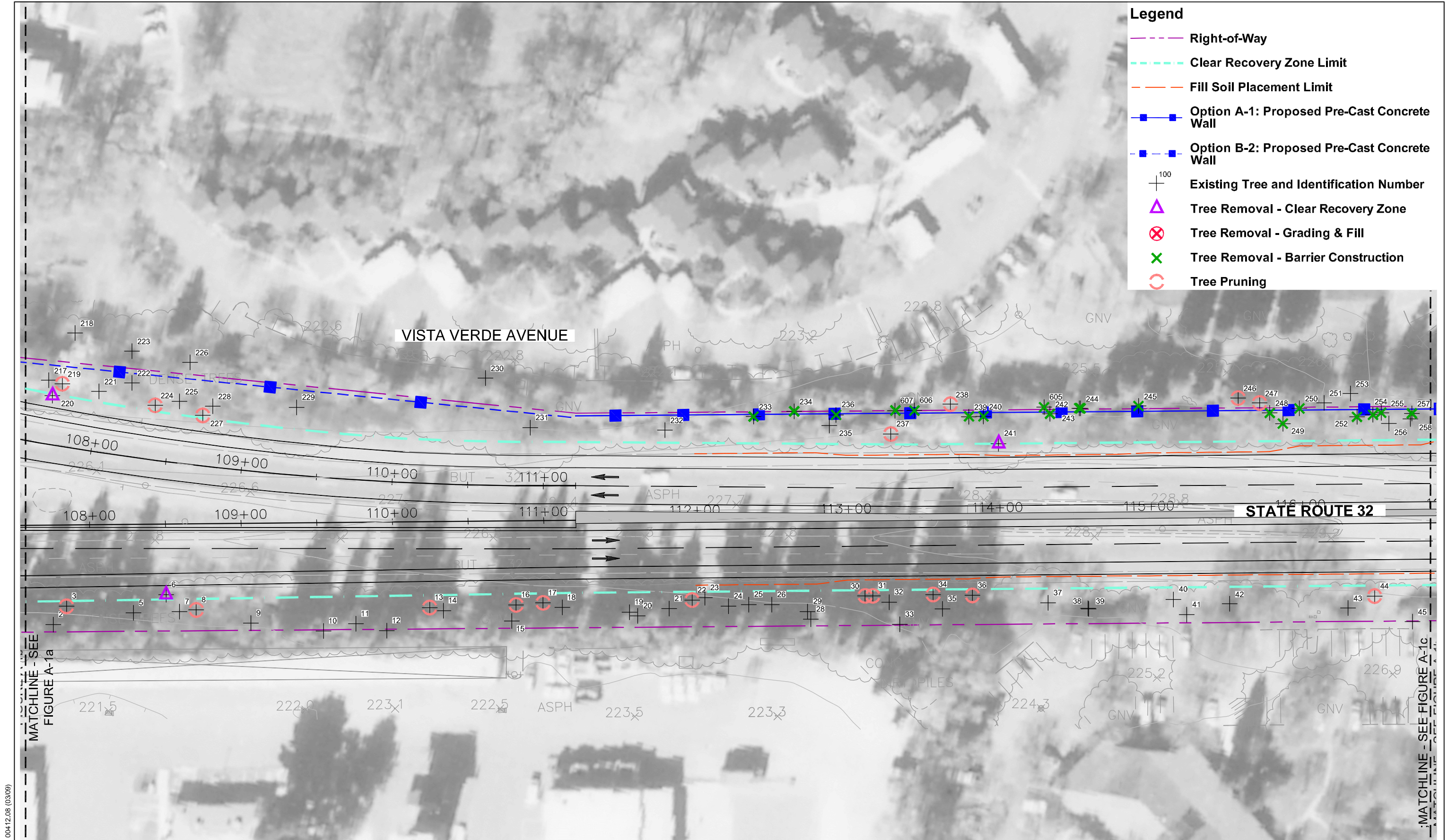
Figure A-1b SR 32 Widening Arborist Report - Pre-Cast Concrete Wall
