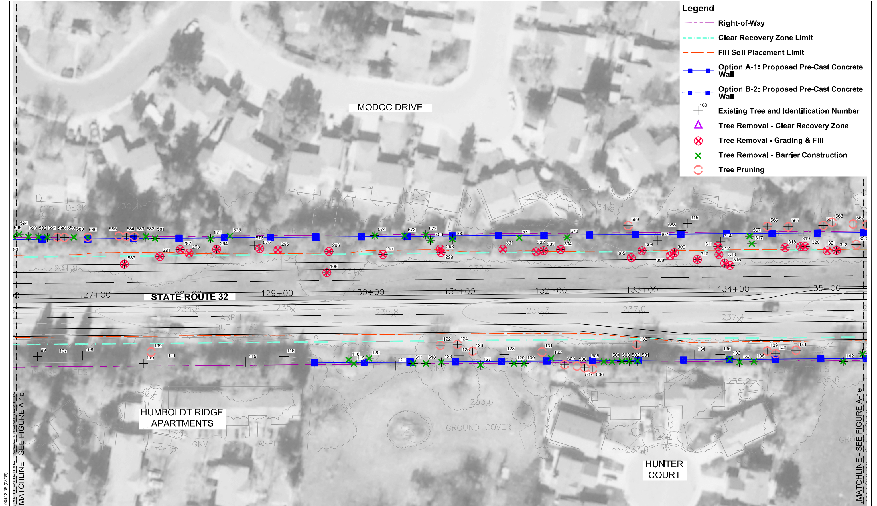
Figure A-1d SR 32 Widening Arborist Report - Pre-Cast Concrete Wall
