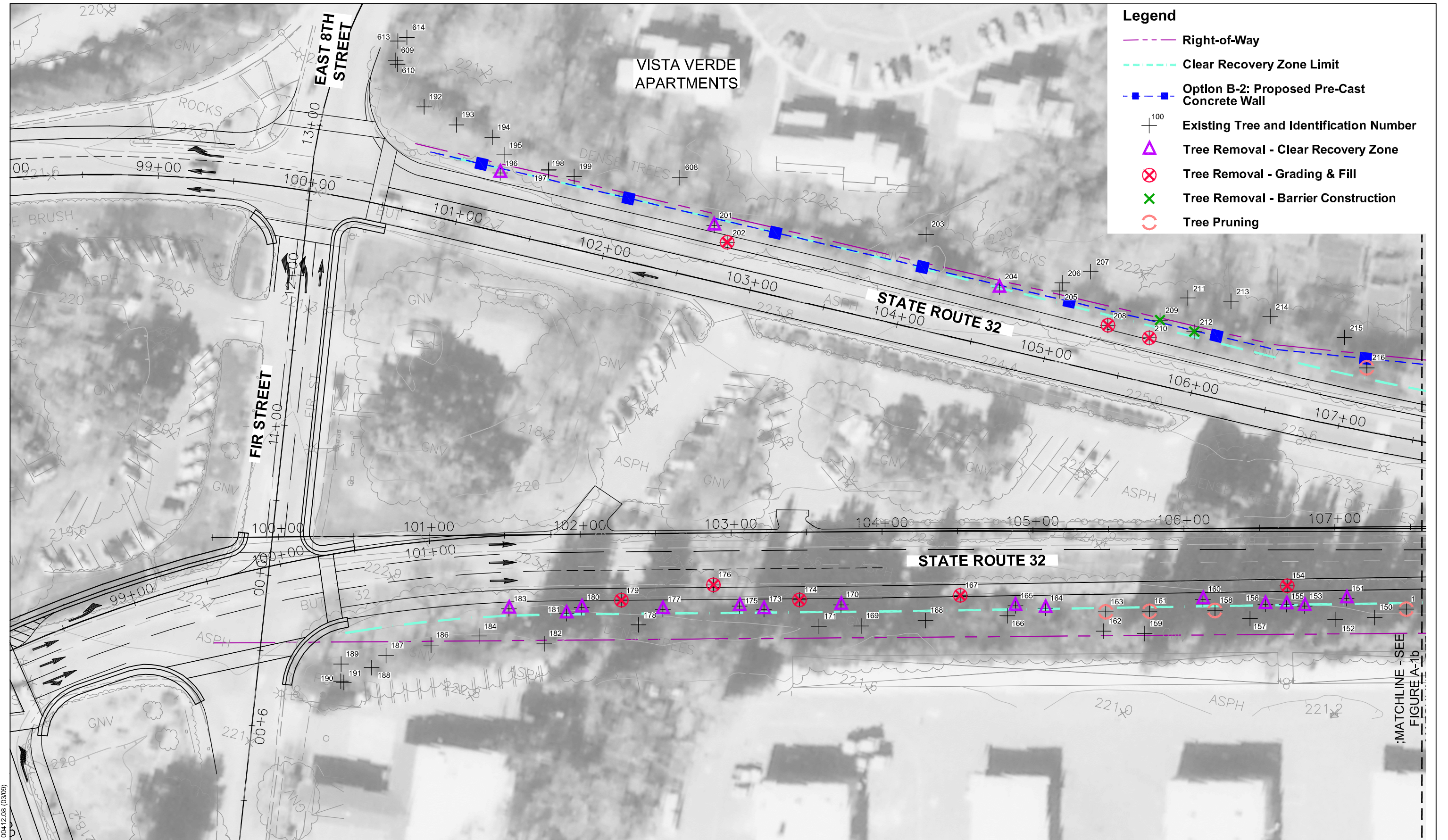
Figure A-1a SR 32 Widening Arborist Report - Pre-Cast Concrete Wall
