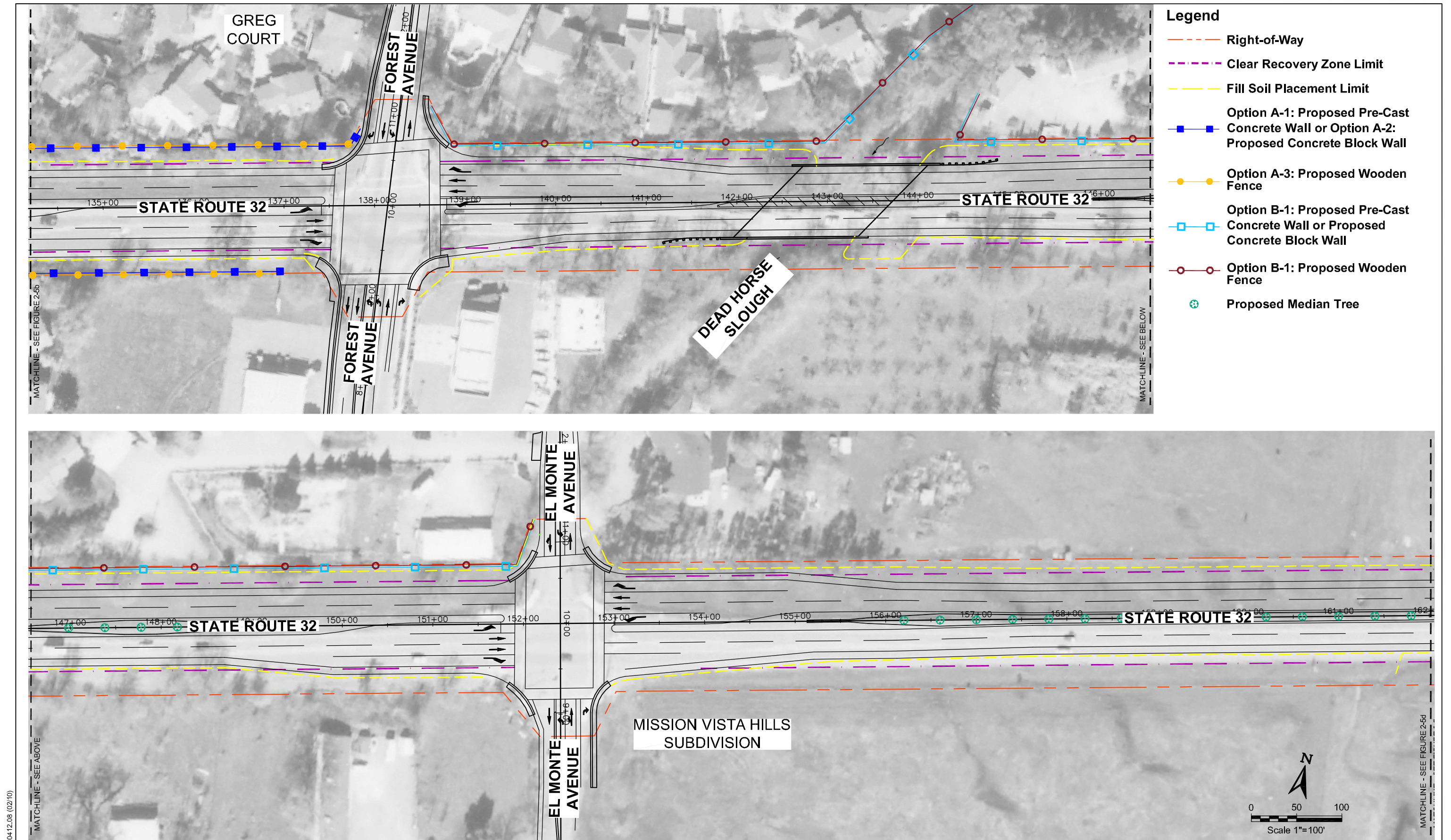
Figure 2-5c Timber Barrier Alternative, including Proposed Sound Barrier
