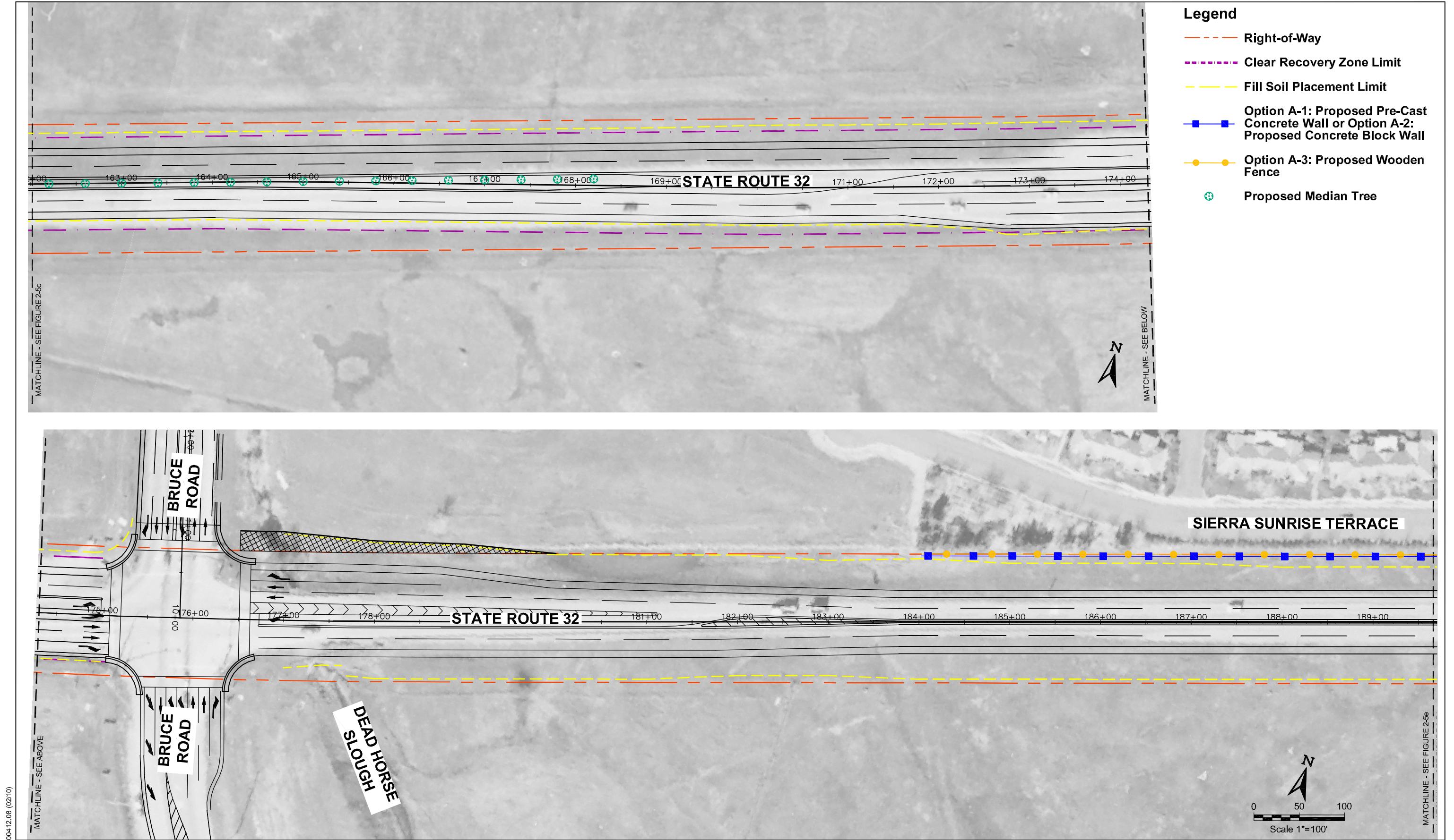
Figure 2-5d Timber Barrier Alternative, including Proposed Sound Barrier
