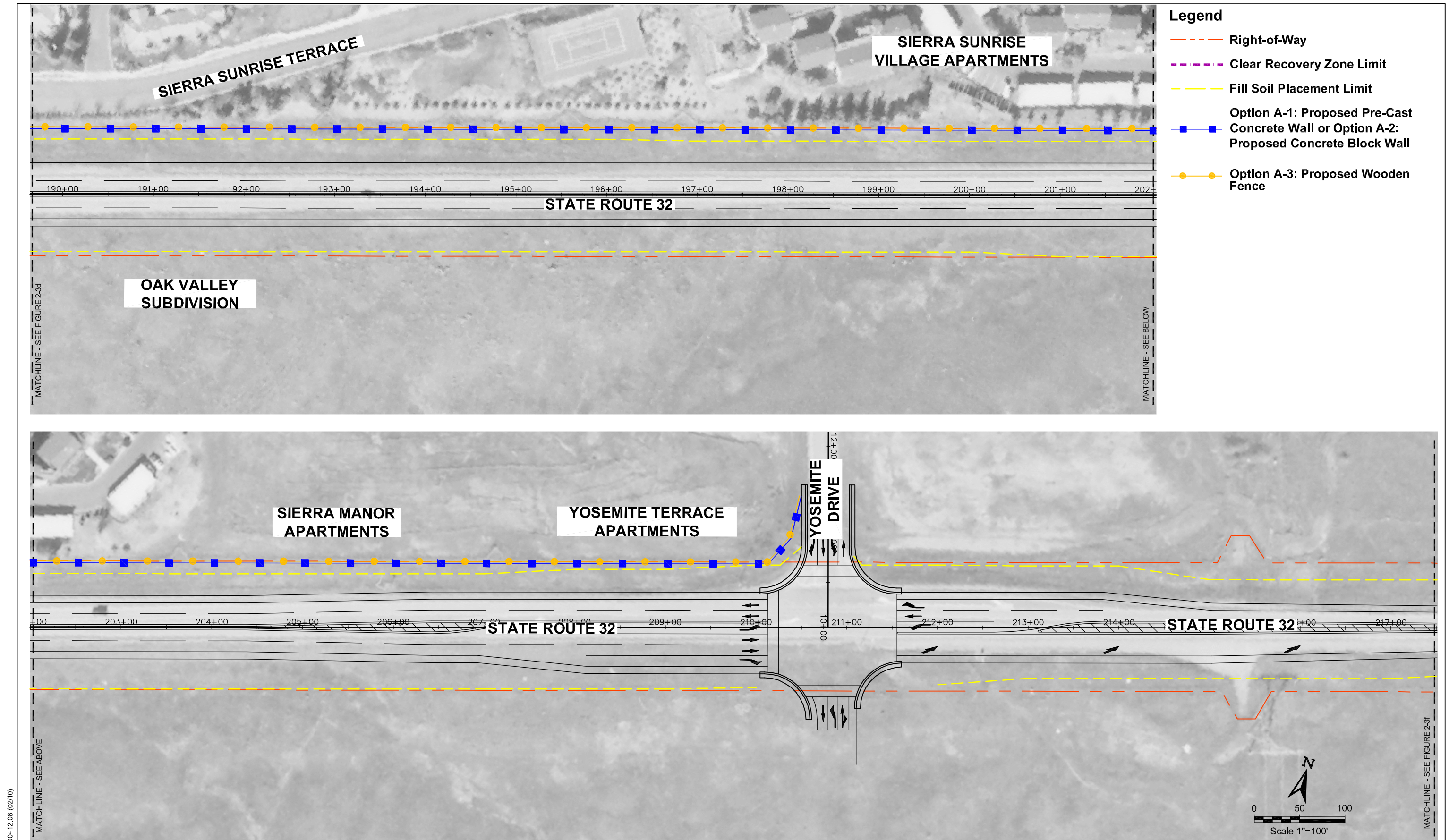
Figure 2-3e Proposed Project, including Proposed Sound Barrier
