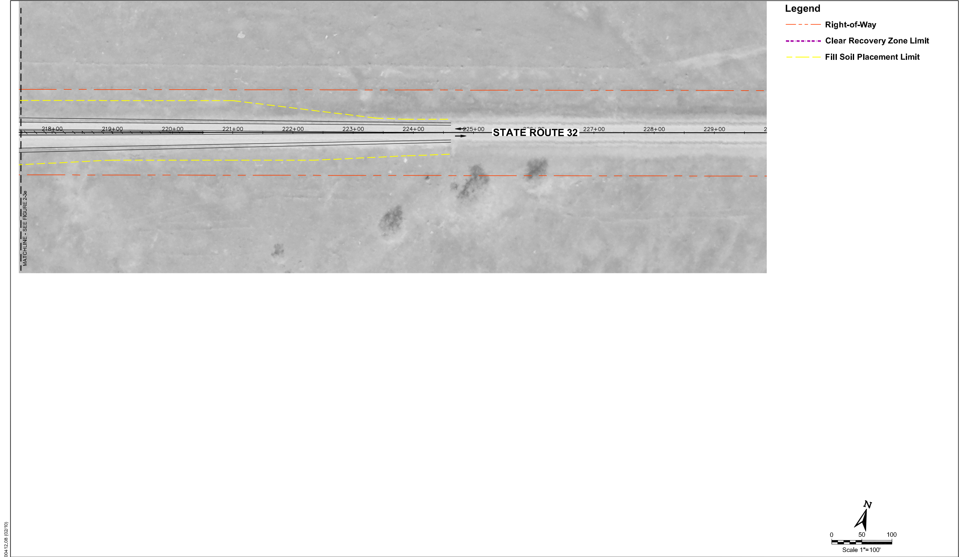
Figure 2-3f Proposed Project, including Proposed Sound Barrier
